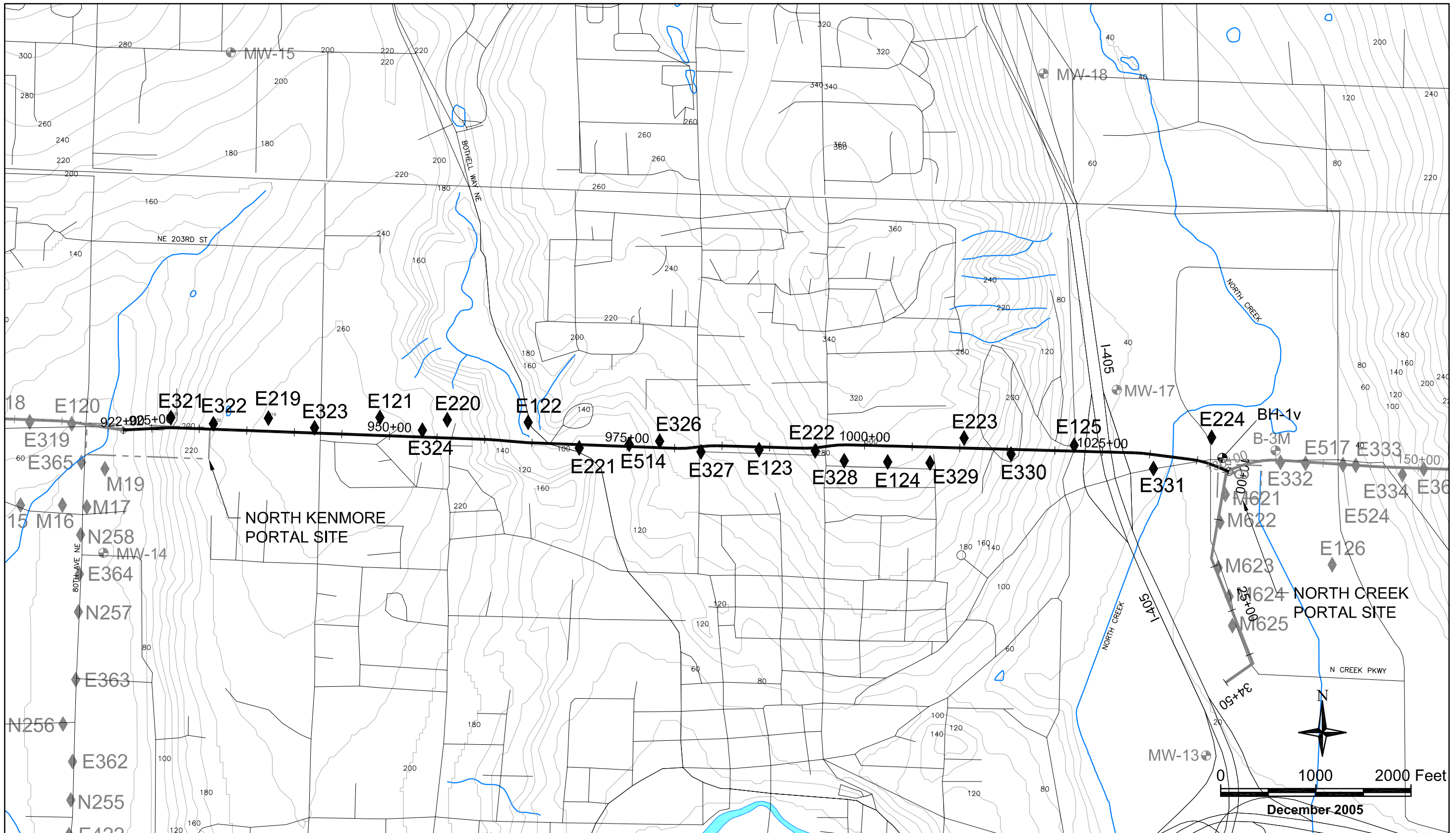
Figure 1-7 Boring Location Plan - Brightwater Tunnel 2 BRIGHTWATER CONVEYANCE GEOTECHNICAL DATA REPORT
